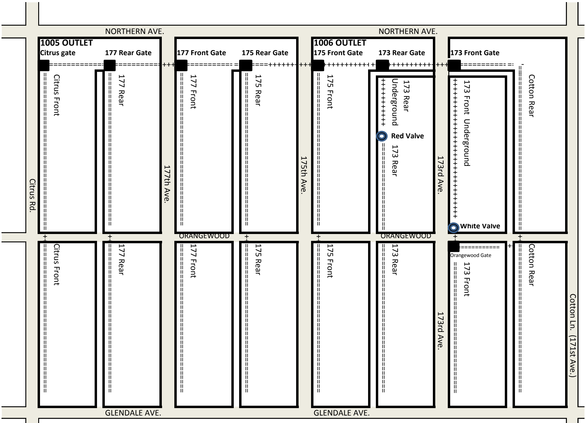
Irrigation Ditch and Gate Map
